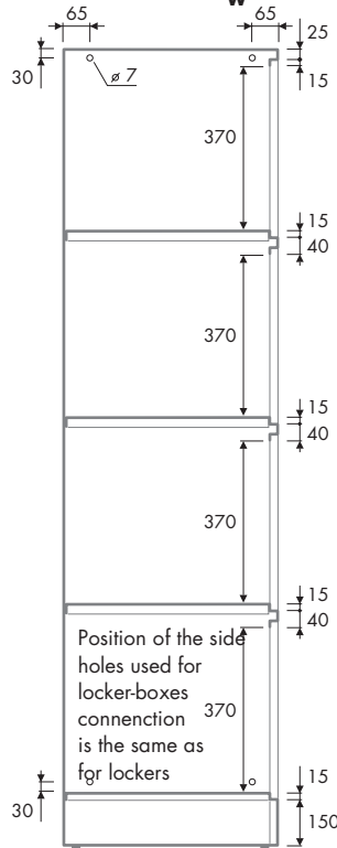
Locker-boxes' side view
